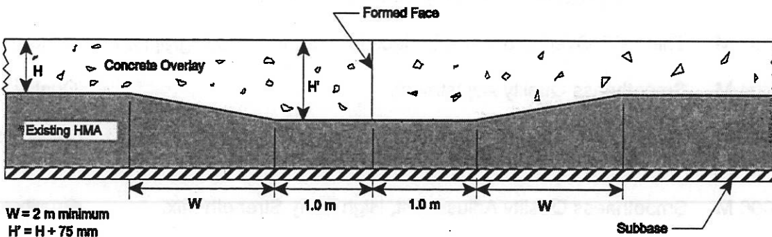
Detail 2 Thickened Edge Transverse Joints at Intersections
